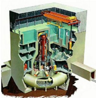
GE BWR Mark 1
